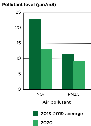
Figure 26. Average levels of fine particulate matter (PM 2.5 ) and nitrogen dioxide (NO 2 ) levels in the UK in the 100 days following the start of the first lockdown, compared with the 2013-19 average
